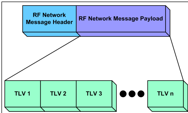
Figure 24-9. RFNM Structure
