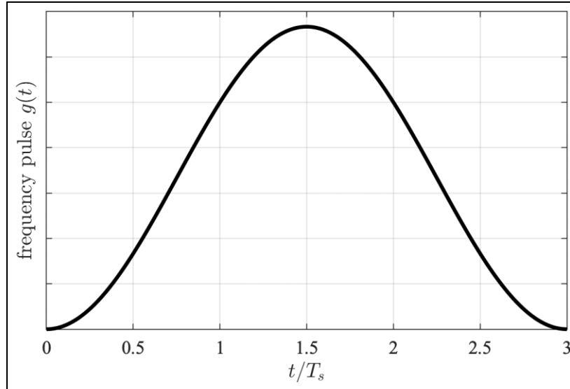
Figure 2-7. The Frequency Pulse for ARTM CPM
