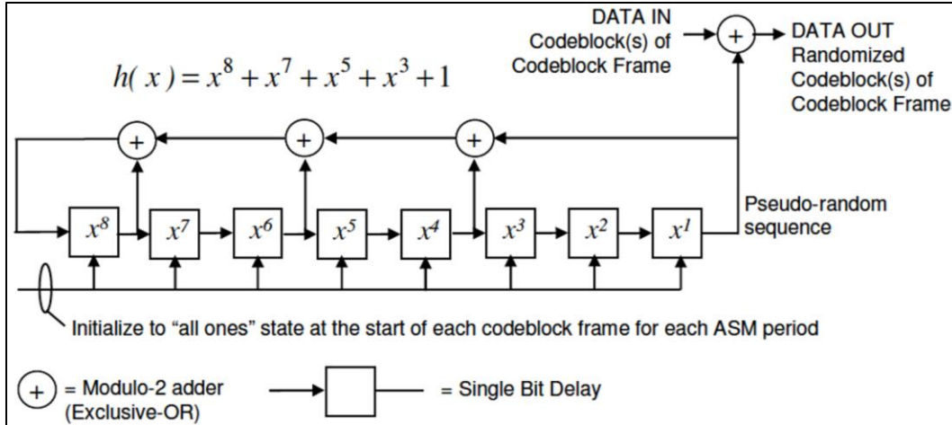
Figure 27-7. Pseudo-Randomizer
