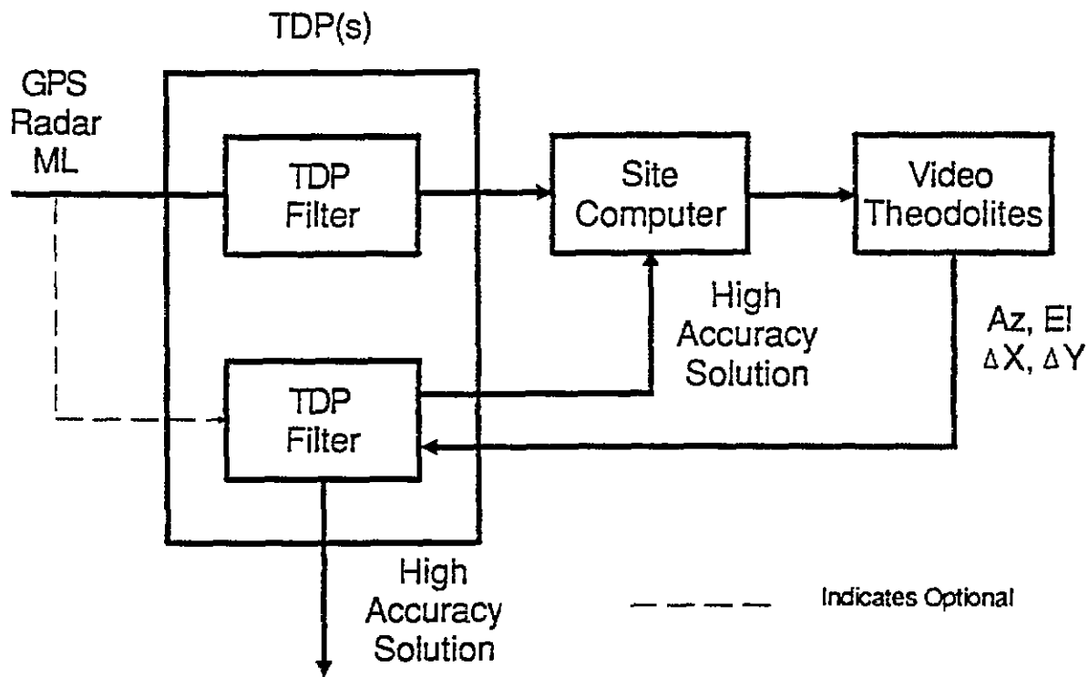
Figure 3-1. Closed Loop Tracker data integration
