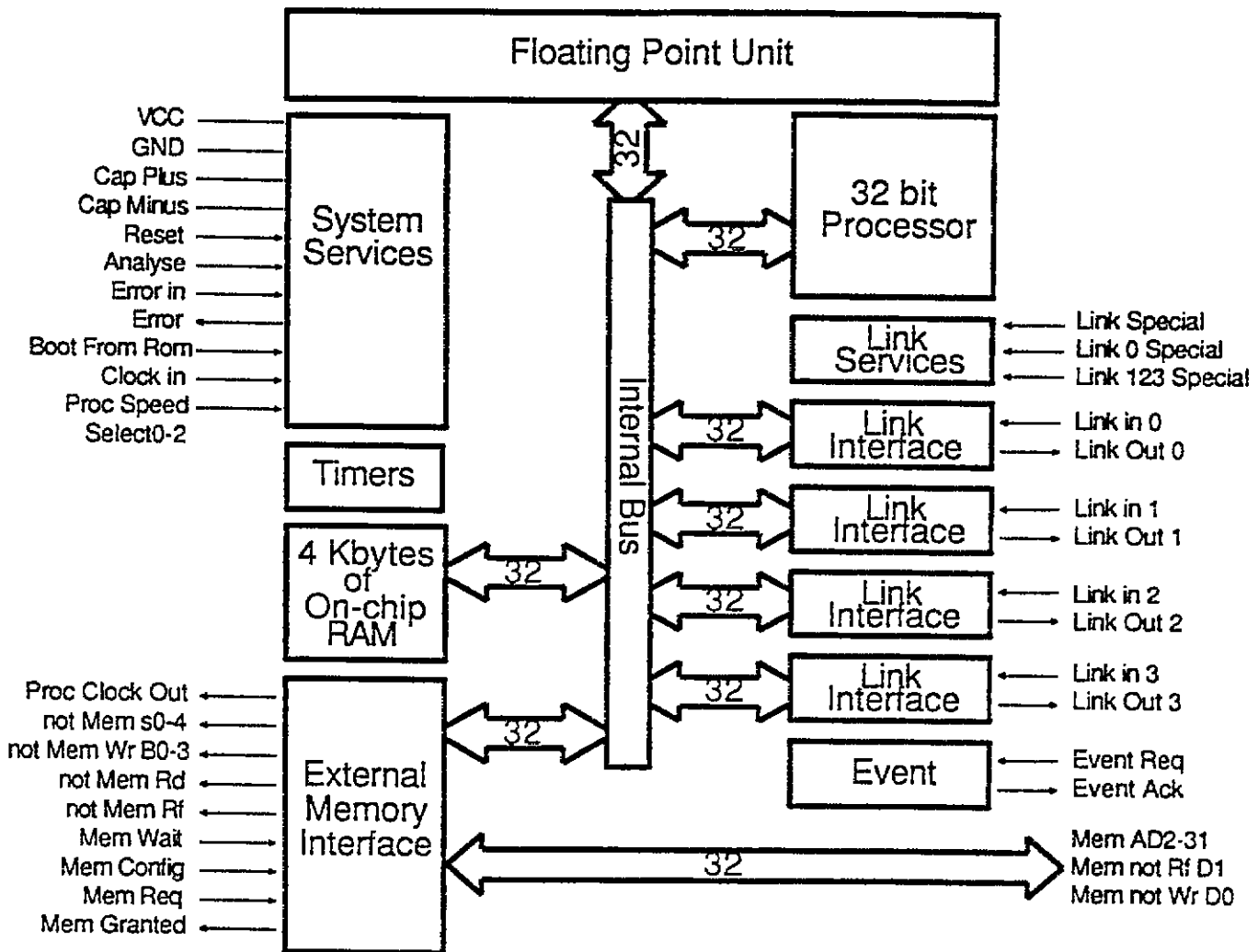
Figure 2-1. Transputer Structure
