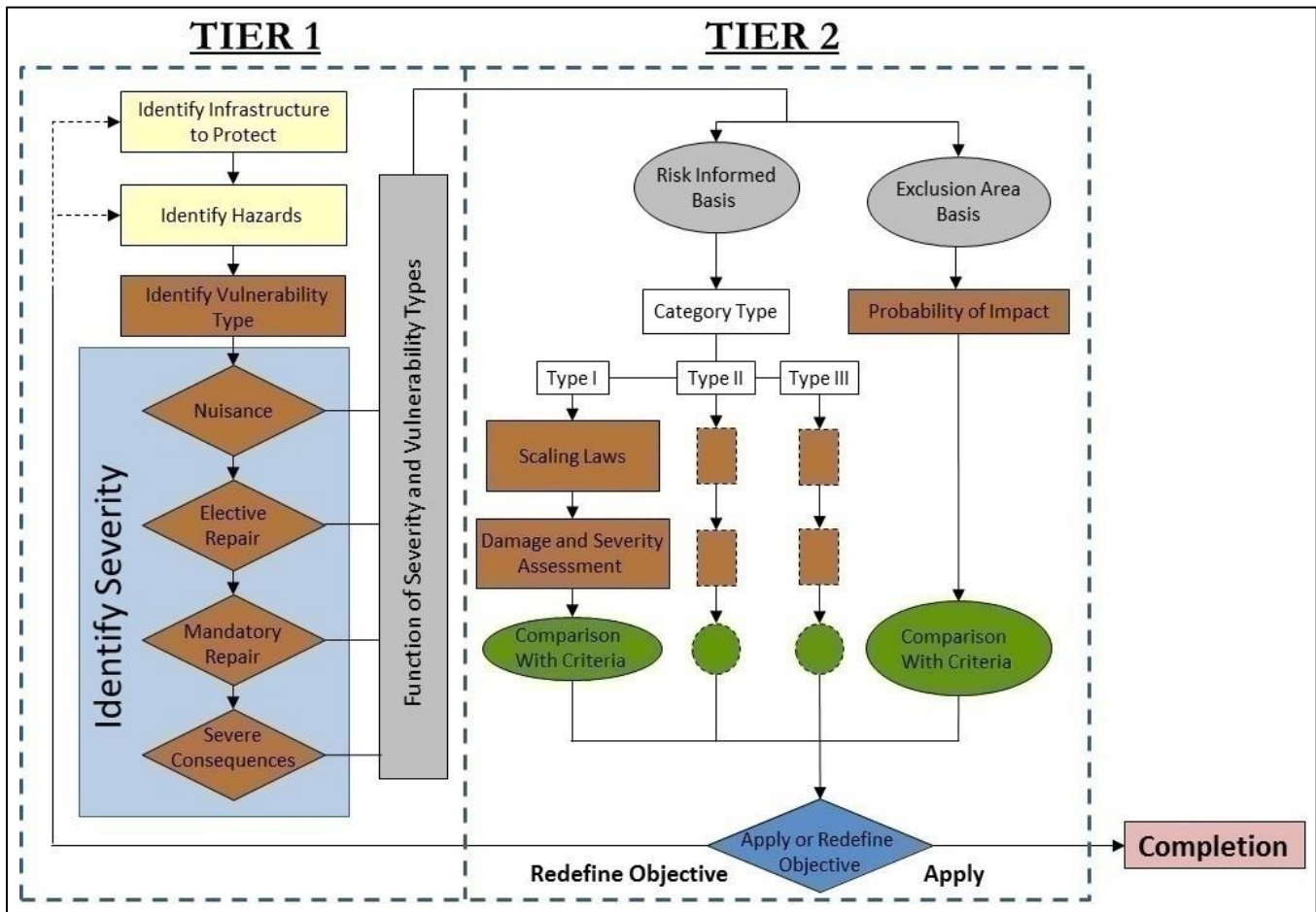
Figure 2-2. Two-Tiered Risk Management Process for Infrastructure
