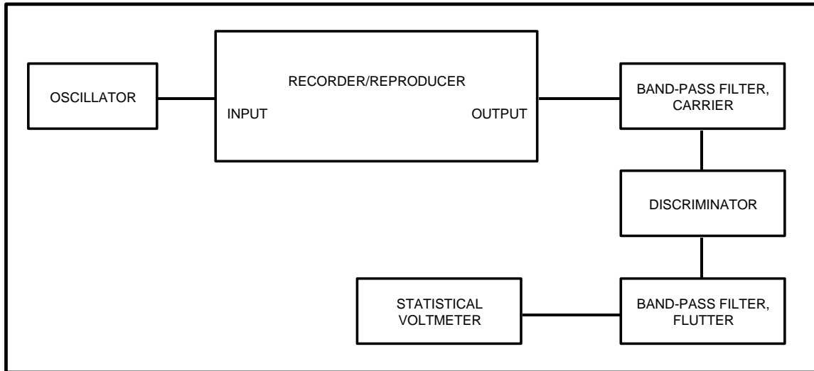
Figure 1-4. Flutter measurement (see test 1.7.1).
