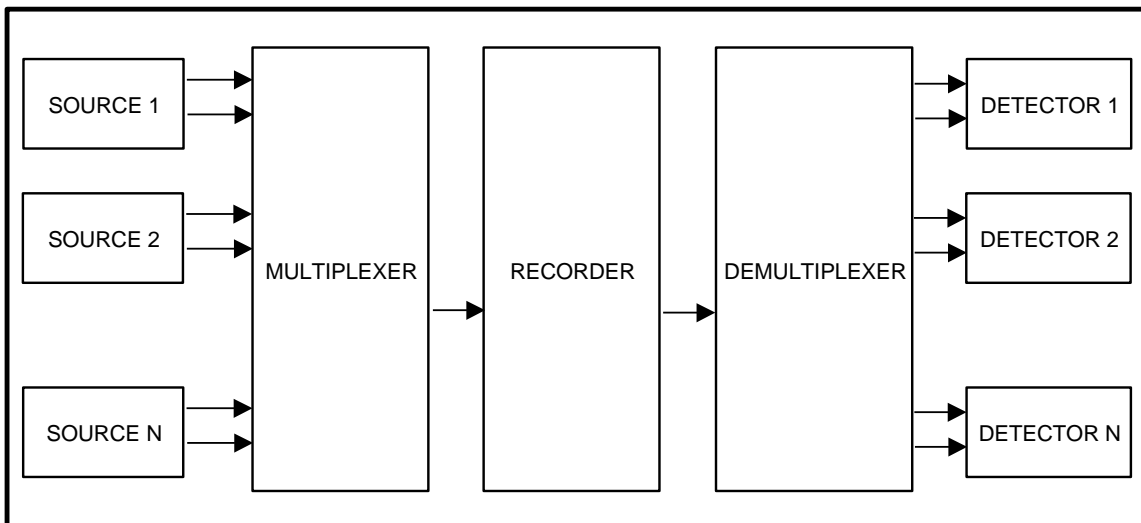
Figure 4-1. Multiplexer/demultiplexer delay measurement.
