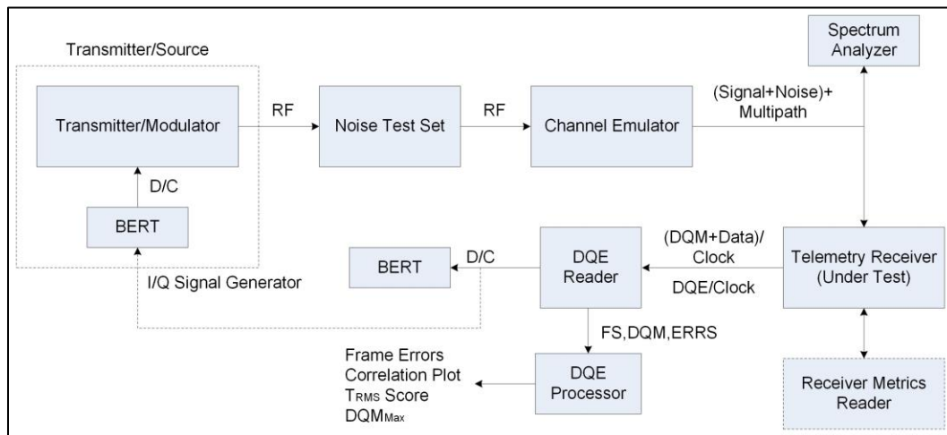
Figure 11-13. Setup for Static 2-ray Multipath Channel Conditions using Channel Emulator
