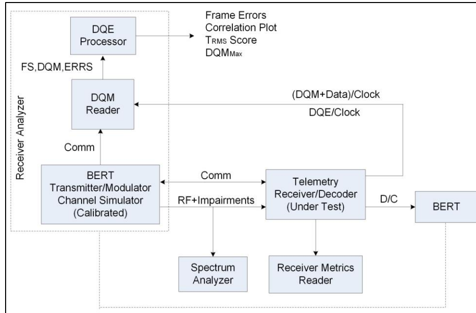
Figure 11-16. Setup for Resynchronization Response using Receiver Analyzer
