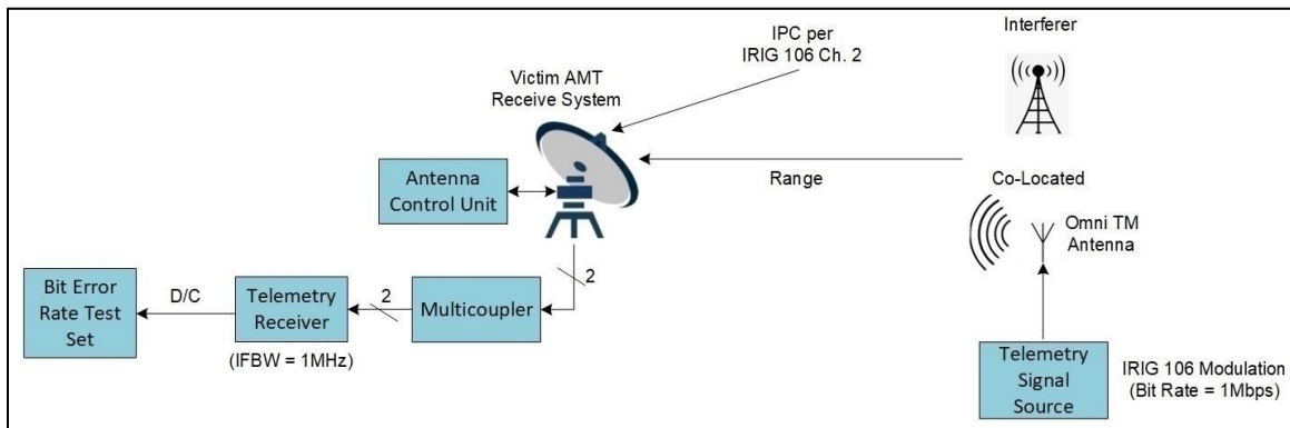
Figure 12-2. Notional Setup for Interference Testing
