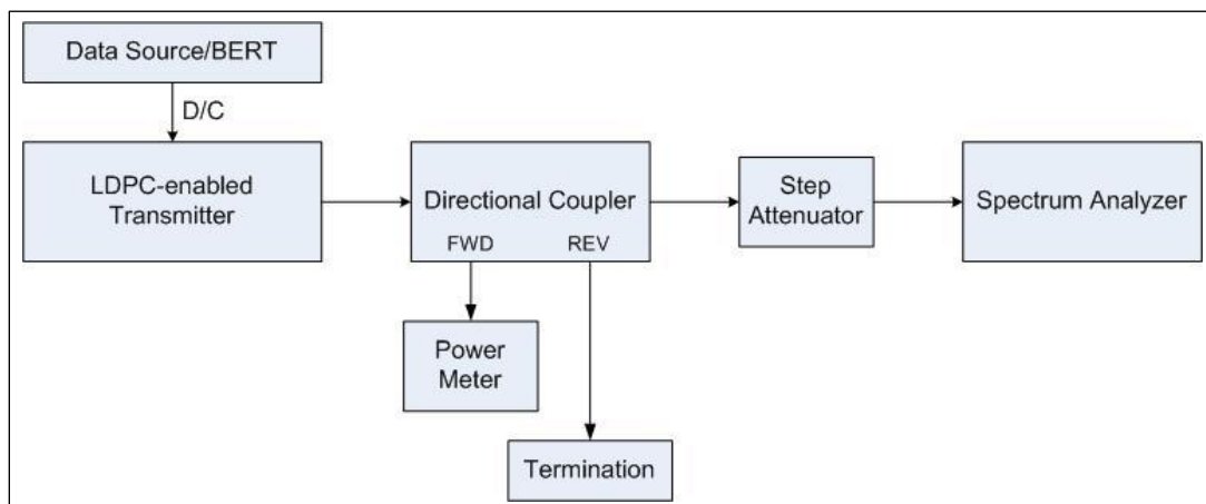
Figure 8-9. Test Setup for 99% Occupied Bandwidth and -25-dBm Bandwidth Test
