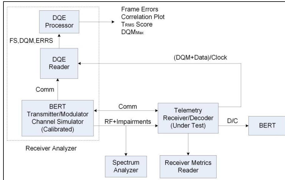
Figure 11-3. Setup using Receiver Analyzer for BER versus BEP Test
