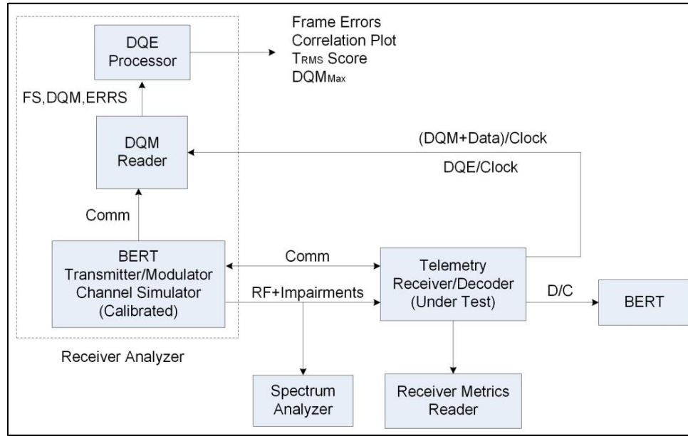
Figure 11-14. Setup for Static 2-ray Multipath Channel Conditions using Channel Emulator
