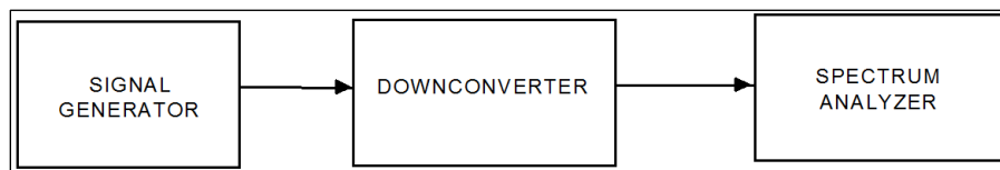
Figure 6-9. Image Rejection Test Setup
