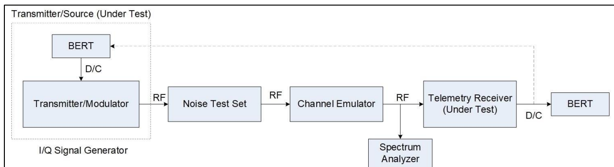
Figure 10-1. Setup using Channel Emulator for 3-Ray Static Multipath Test
