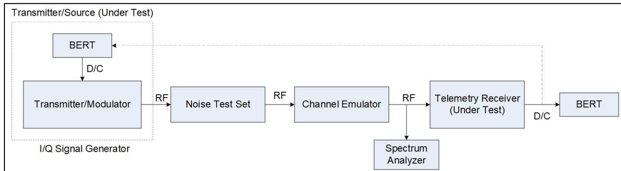
Figure 10-4. Setup using Channel Emulator for 2-ray Static Multipath Test
