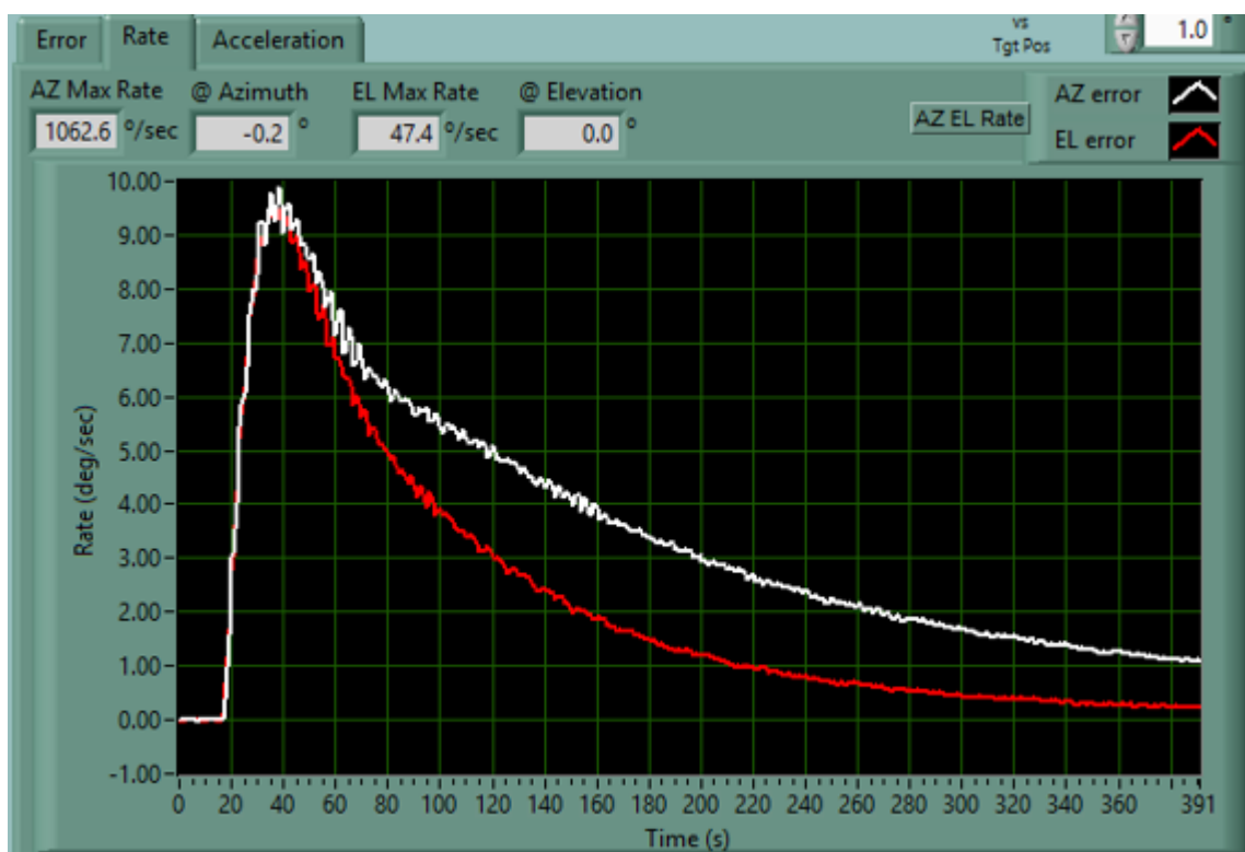
Figure 1-21. Example MIV Antenna Angular Rates
