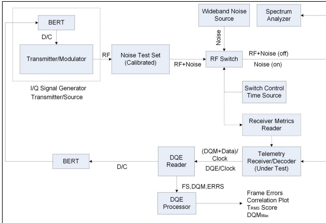
Figure 11-15. Setup for Resynchronization Response using Noise Test Set
