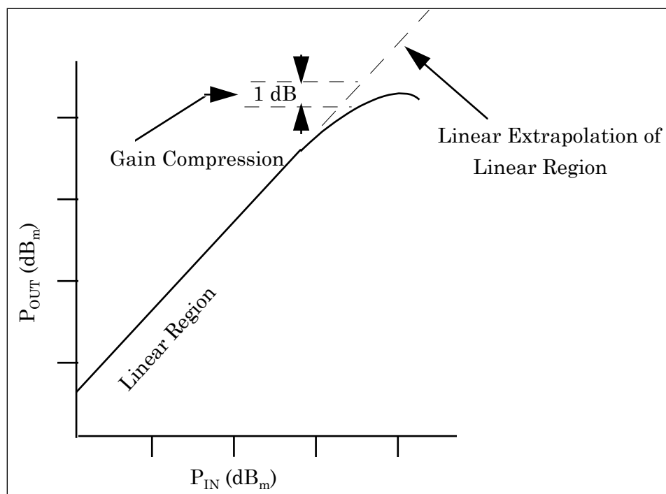
Figure 2-2. Amplifier Gain Compression
