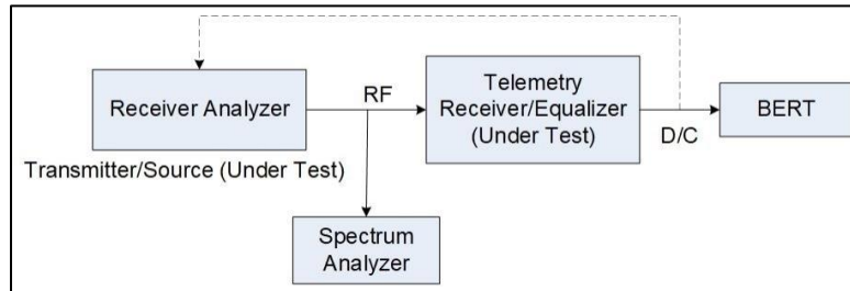
Figure 10-7. Setup using Receiver Analyzer for Dynamic Channel Multipath Test
