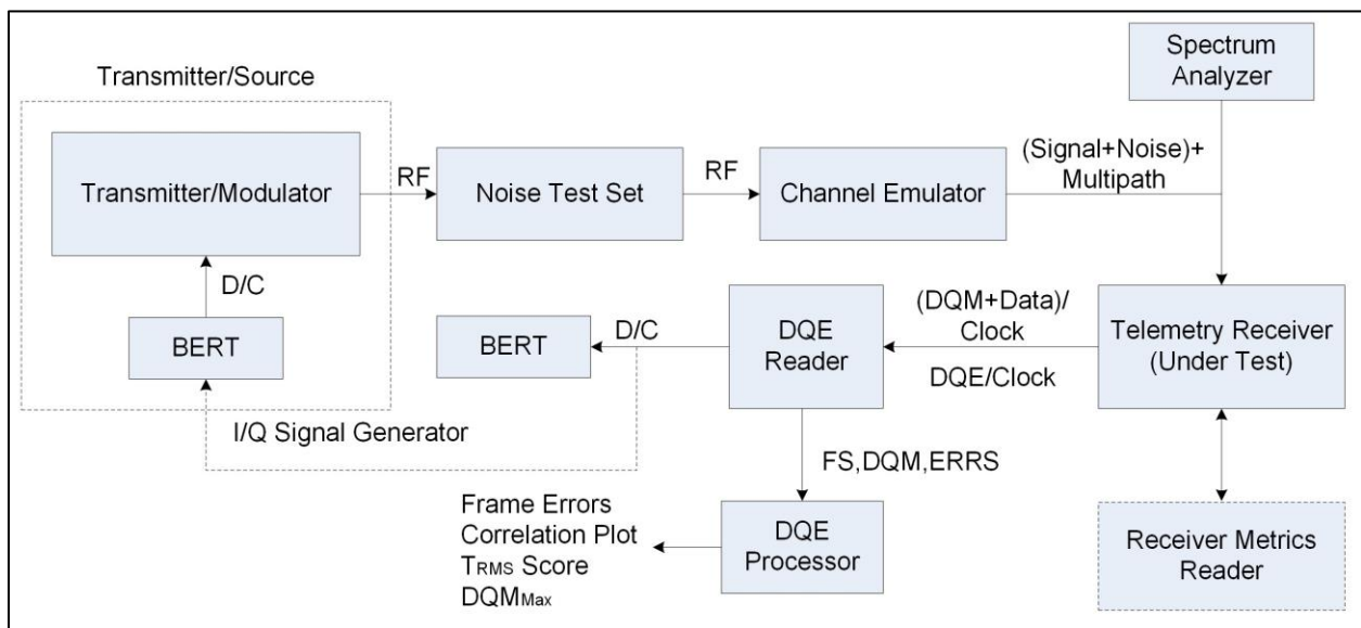
Figure 11-11. Setup for Static 3-ray Multipath Channel Conditions using Channel Emulator
