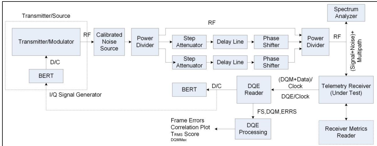
Figure 11-10. Setup for Static 3-ray Multipath Channel Conditions using Discrete Components
