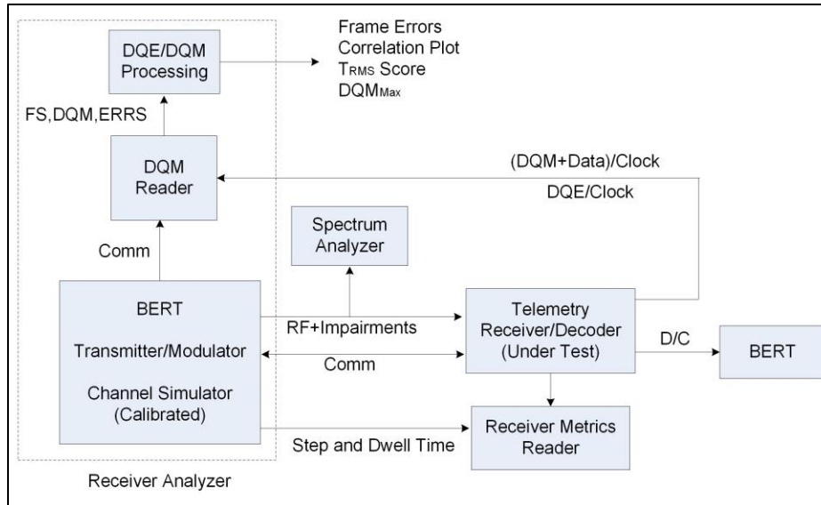
Figure 11-6. Setup for Step and Dwell Test using Receiver Analyzer
