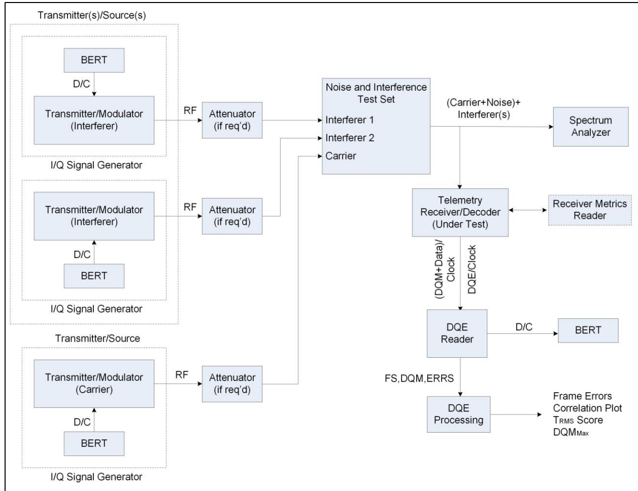
Figure 11-8. Setup for ACI Test using Noise and Interference Test Set
