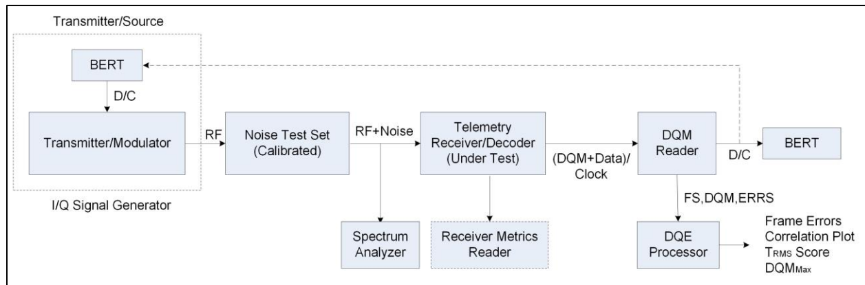
Figure 11-2. Setup using Noise Test Set for BER versus BEP Test
