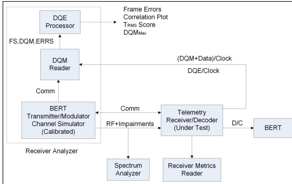
Figure 11-9. Setup for ACI Test using Receiver Analyzer
