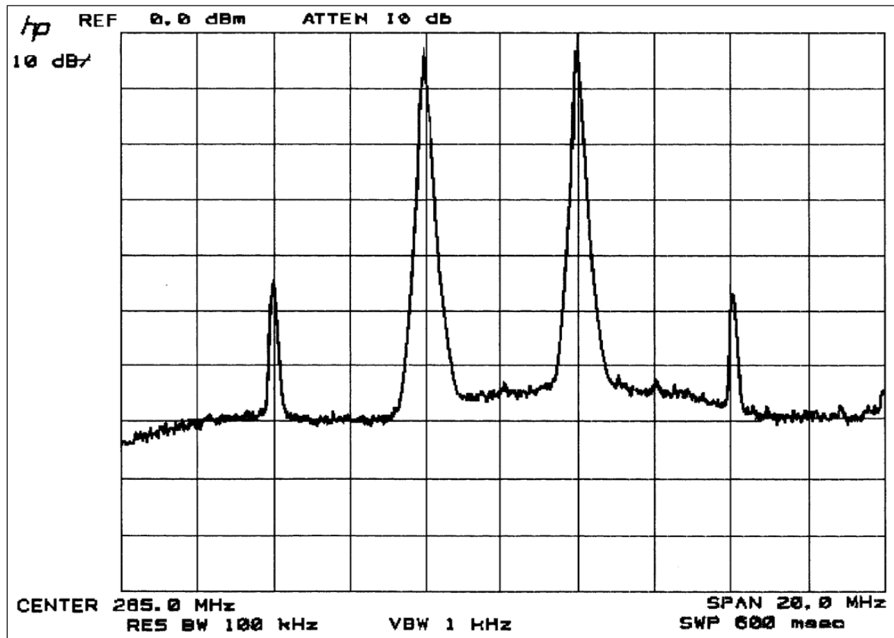
Figure 6-4. Downconverter Intermodulation Products
