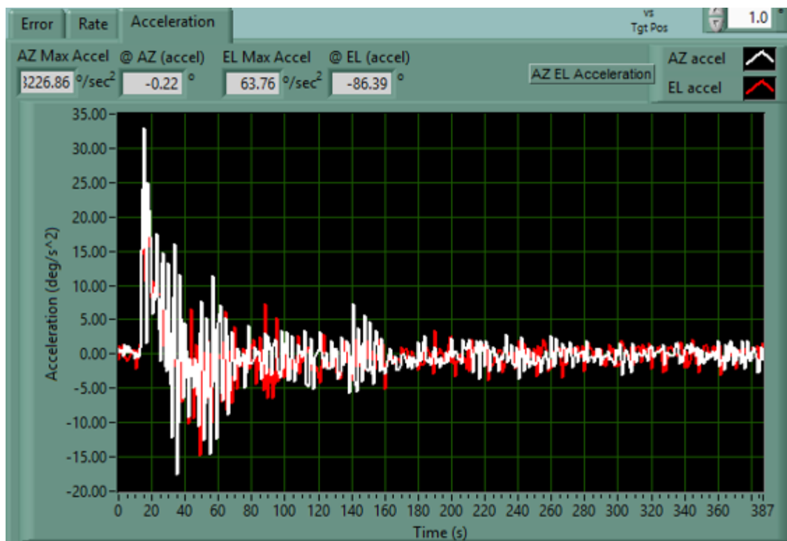
Figure 1-22. Example Maximum MIV Antenna Acceleration
