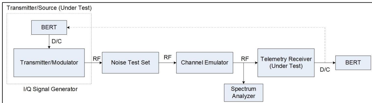
Figure 10-6. Setup using Channel Emulator for Dynamic Channel Multipath Test
