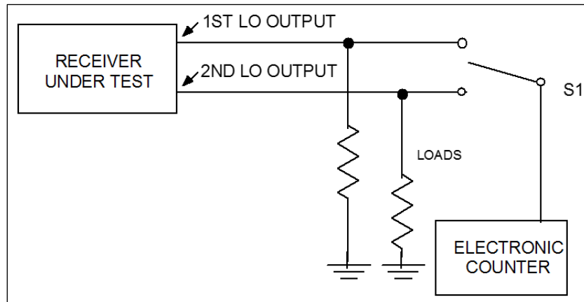
Figure 4-12. Local Oscillator Stability Test
