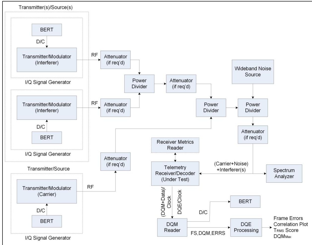
Figure 11-7. Setup for ACI Test using Discrete Components
