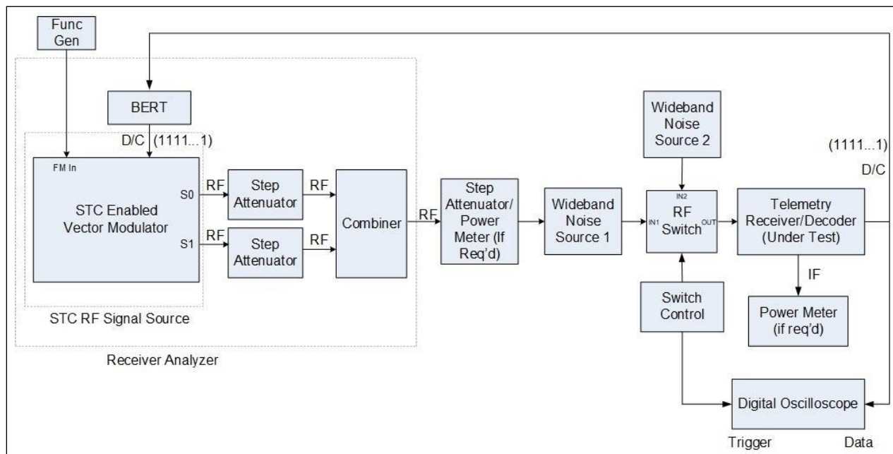
Figure 9-4. Test Setup for Receiver/Decoder Acquisition and Flat Fade Recovery
