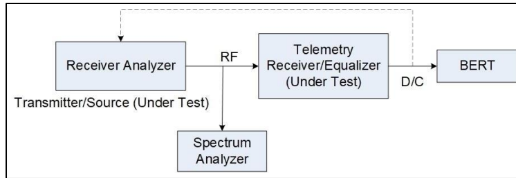
Figure 10-5. Setup using Receiver Analyzer for 2-ray Static Multipath Test
