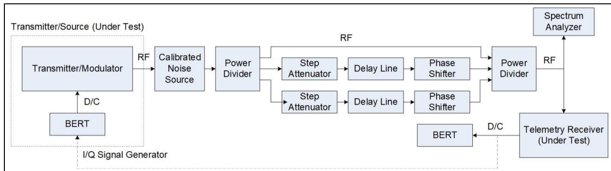
Figure 10-3. Setup using Discrete RF Components for 3-Ray Static Multipath Test
