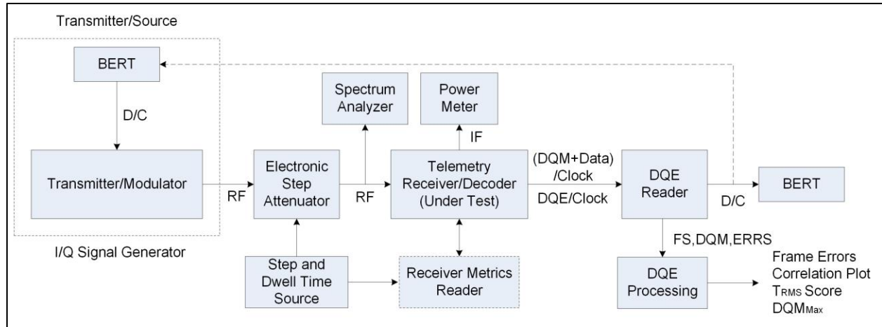
Figure 11-4. Setup for Step and Dwell Testing using Step Attenuator/Power Meter
