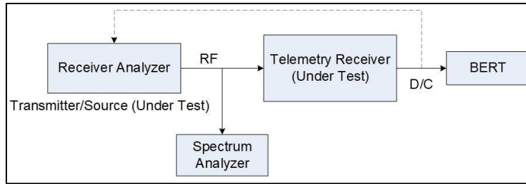
Figure 10-2. Setup using Receiver Analyzer for 3-Ray Static Multipath Test
