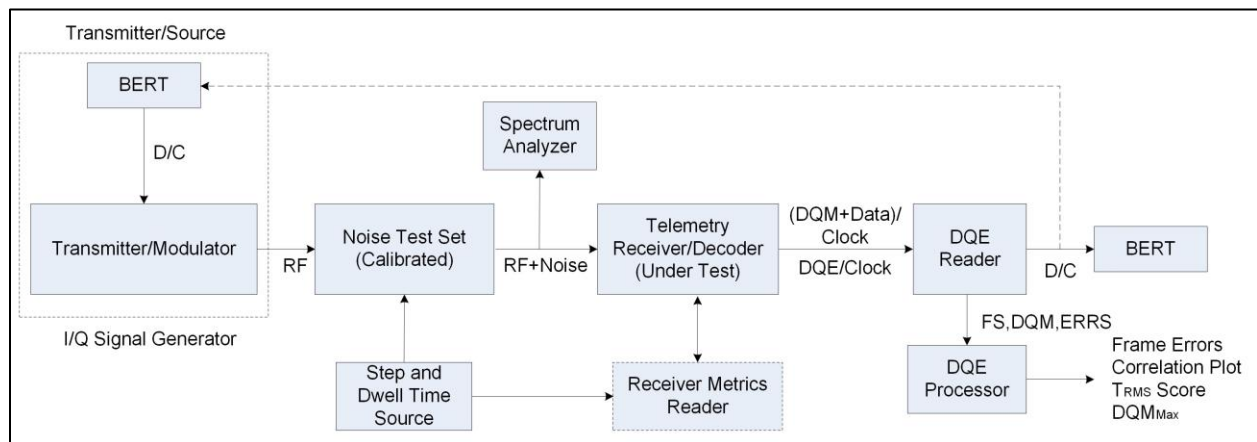
Figure 11-5. Setup for Step and Dwell Test using Noise Test Set
