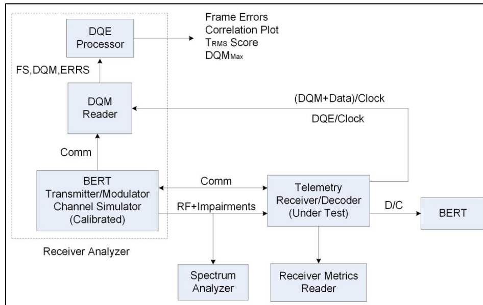
Figure 11-12. Setup for Static 3-ray Multipath Channel Conditions using Receiver Analyzer
