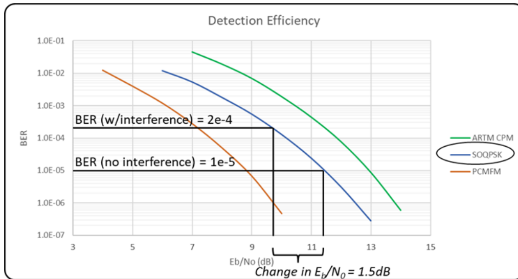
Figure 12-1. Graphical Analysis Example - Determine E_b/N_0 Degradation
