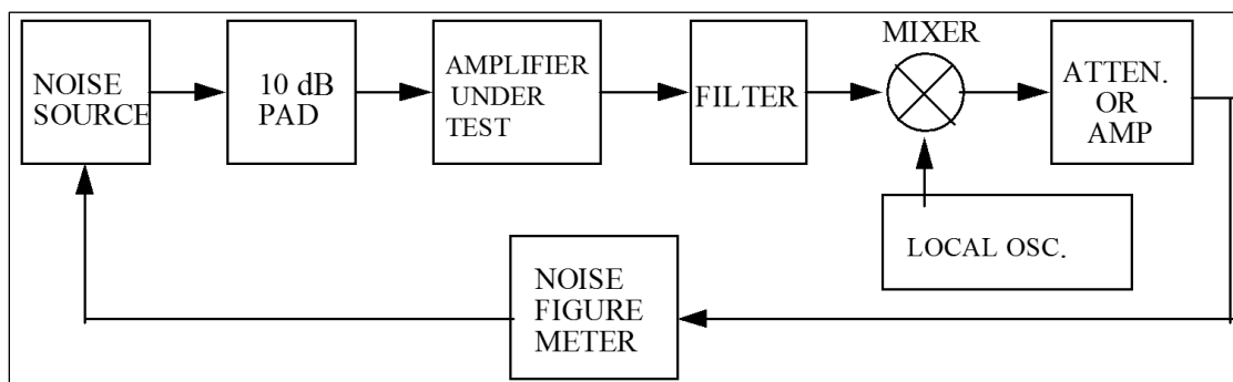
Figure B-4. Noise Figure using Filter, Mixer, and Oscillator
