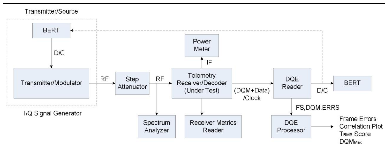
Figure 11-1. Setup for Step Attenuator/Power Meter for BER versus BEP Test
