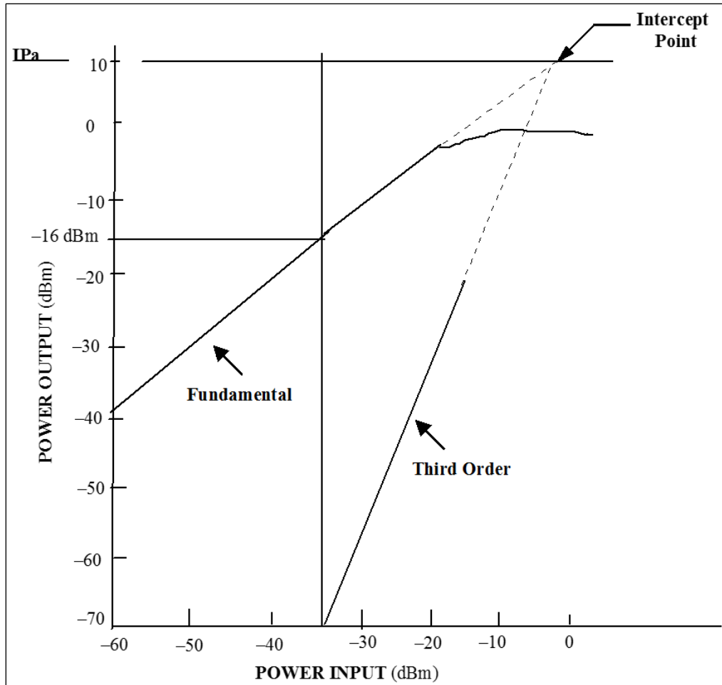
Figure 2-7. Graphical Illustration of Intercept Point
