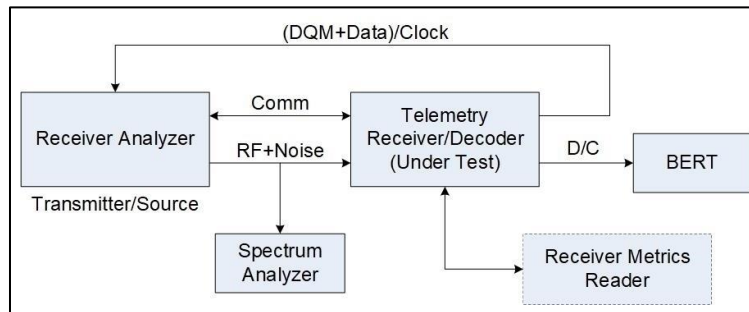
Figure 11-3. Setup using Receiver Analyzer for BER versus BEP Test
