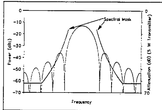
Figure A-9. 1000 kbps OQPSK signal (sinusoidal weighting) and spectral mask.
