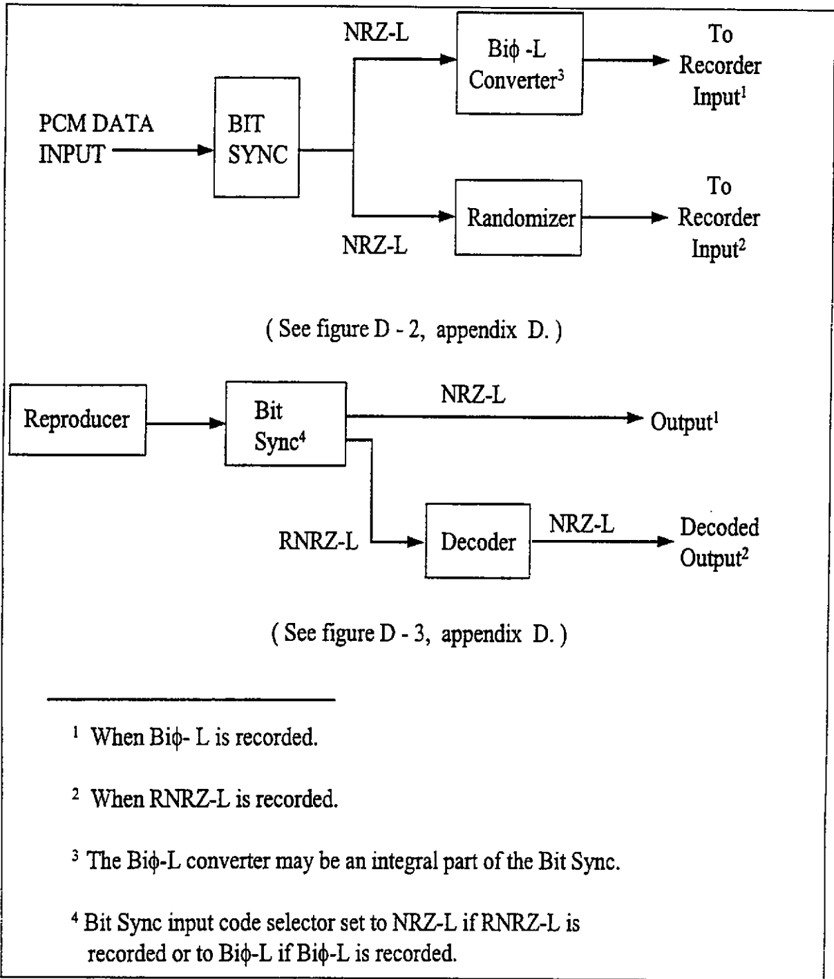
Figure 6-5. Serial high-density digital record and reproduce.
