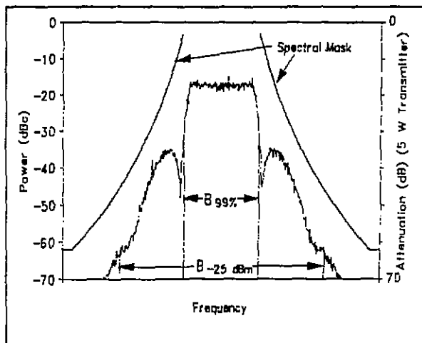
Figure A-7. 1000 kbps RNRZ PCM/FM signal and spectral mask (frequency span = 5 MHz).
