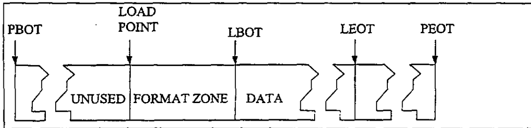
Figure 6-13. Tape cartridge layout.
