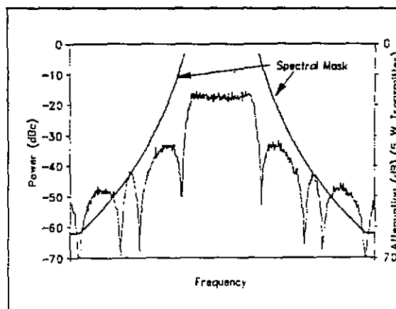
Figure A-8. Unfiltered 1000 kbps RNRZ PCM/FM signal and spectral mask.
