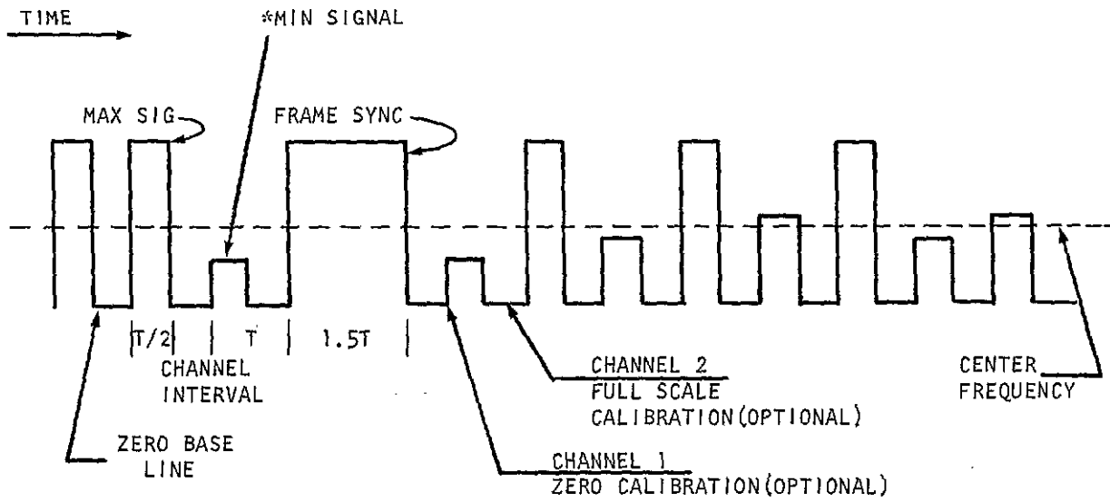
*20 to 25 percent deviation reserved for pulse synchronization is recommended FIGURE 2 50 PERCENT DUTY CYCLE PAM WITH AMPLITUDE SYNCHRONIZATION
