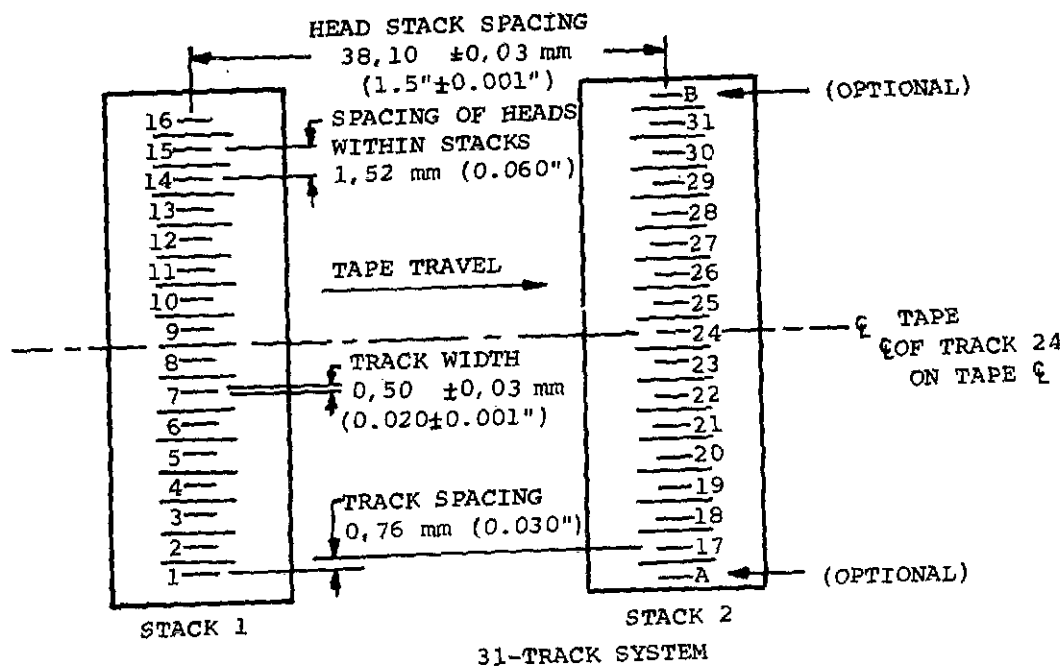
FIGURE 8. PCM HEAD CONFIGURATION.
