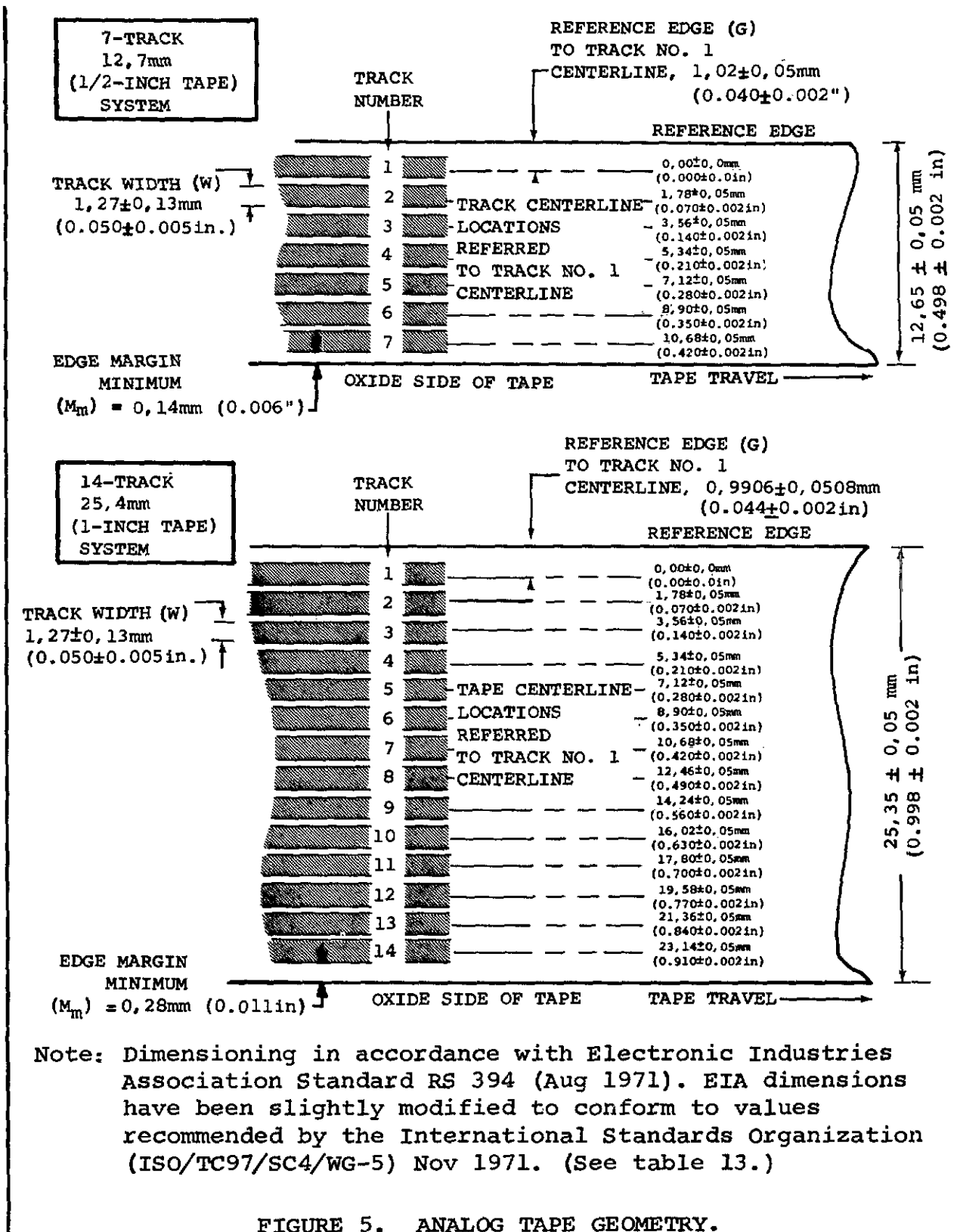
FIGURE 5. ANALOG TAPE GEOMETRY.
