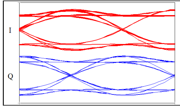
Figure A-17. FQPSK-B I & Q Eye Diagrams (at Input to IQ Modulator)
