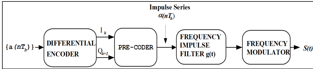
Figure 2-3. SOQPSK Transmitter
