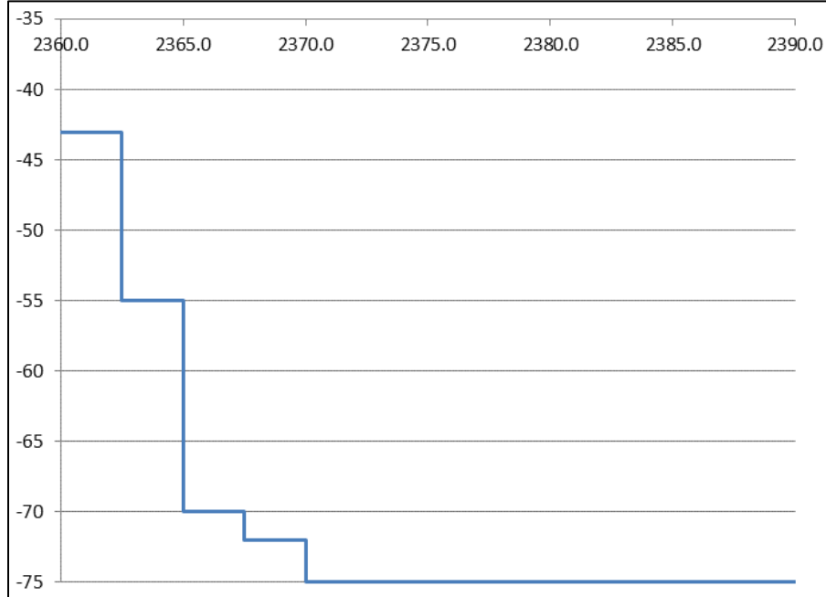
Figure F-5. FCC Emission Mask for the WCS OOB E Band from 2360 – 2390 MHz
