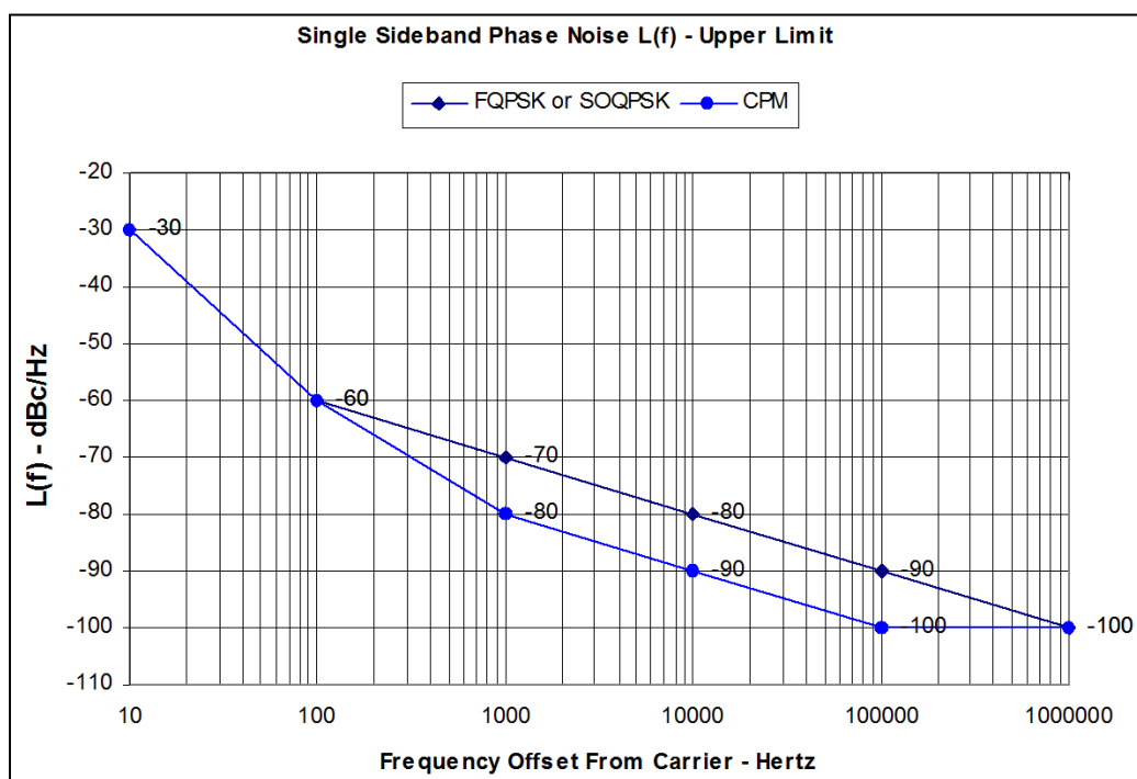
Figure 2-5. Continuous Single-Sideband Phase Noise Power Spectral Density
