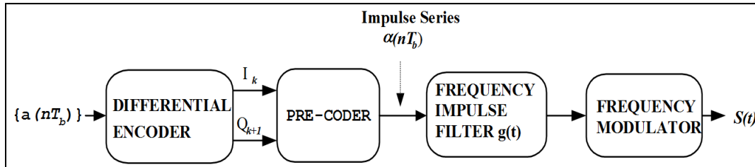
Figure 2-3. SOQPSK Transmitter
