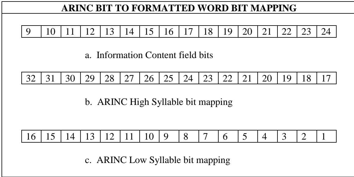
Figure 8-7. ARINC bit to formatted word bit mapping.
