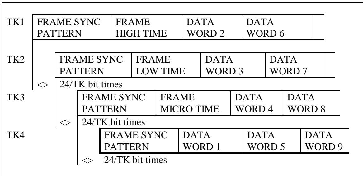
Figure 8-3. Multiple tape track spread format (4-track spread example).
