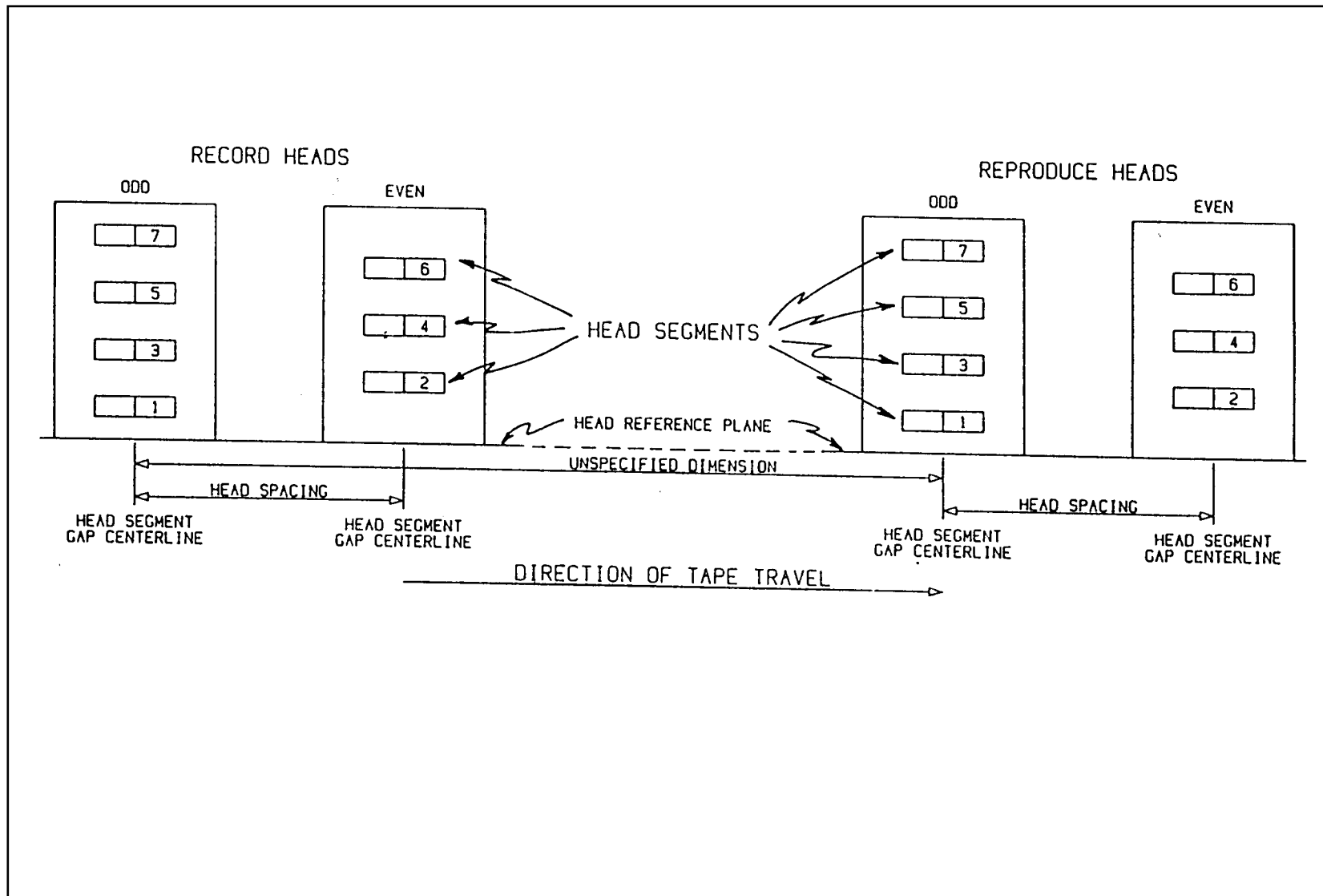
Figure D-1. Record and reproduce head and head segment identification and location (7-track interlaced system).
