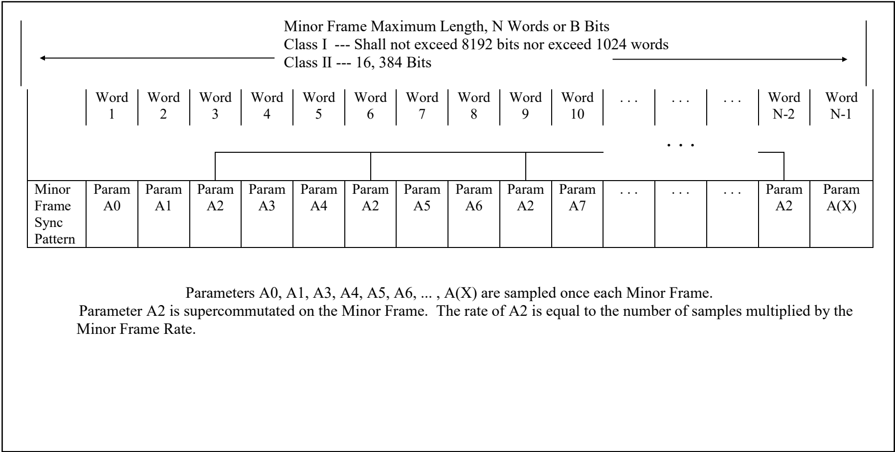
Figure C-4. Major Frame Length = Minor Frame Maximum Length.
