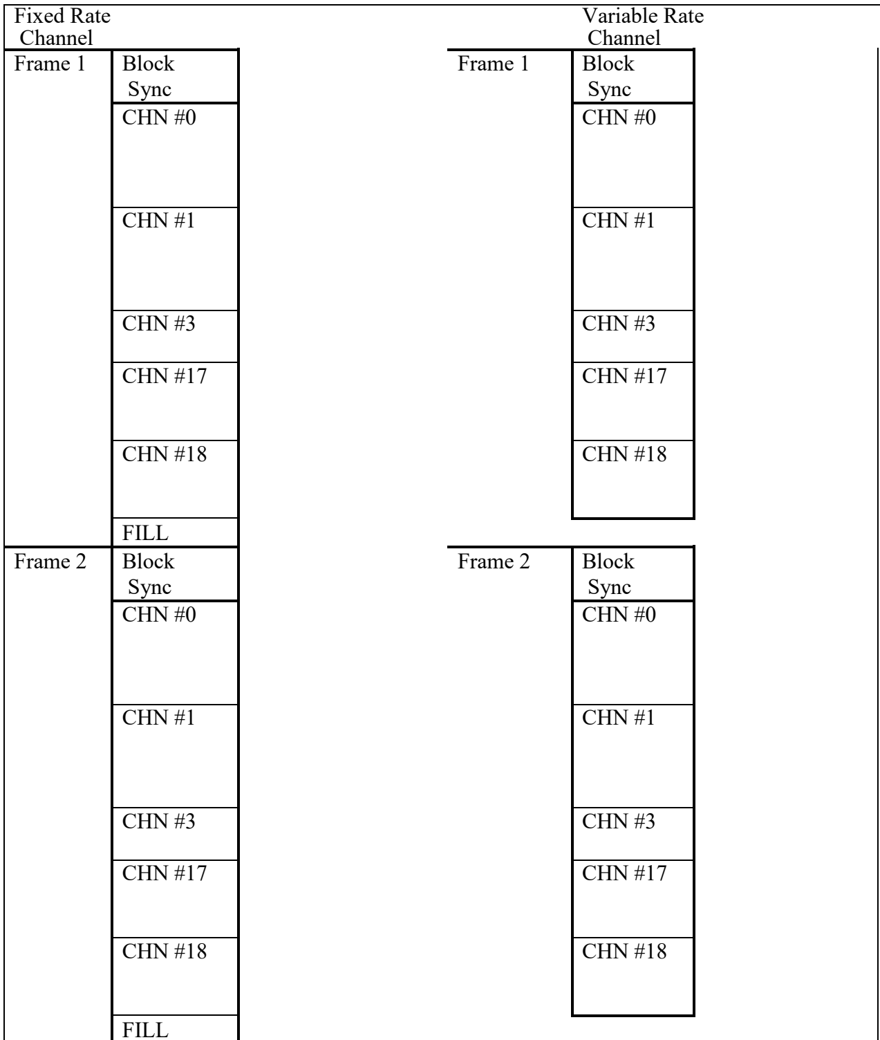
Figure G-5. Submux aggregate format.
