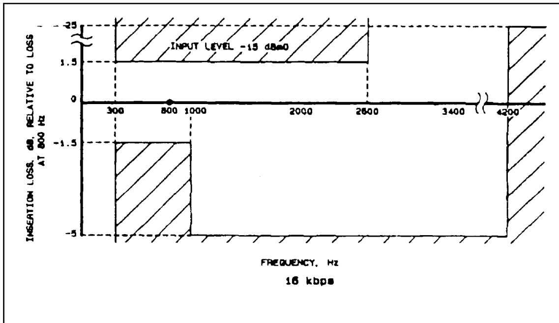
Figure F-4a. Insertion loss versus frequency for CVSD (16 kbps).
