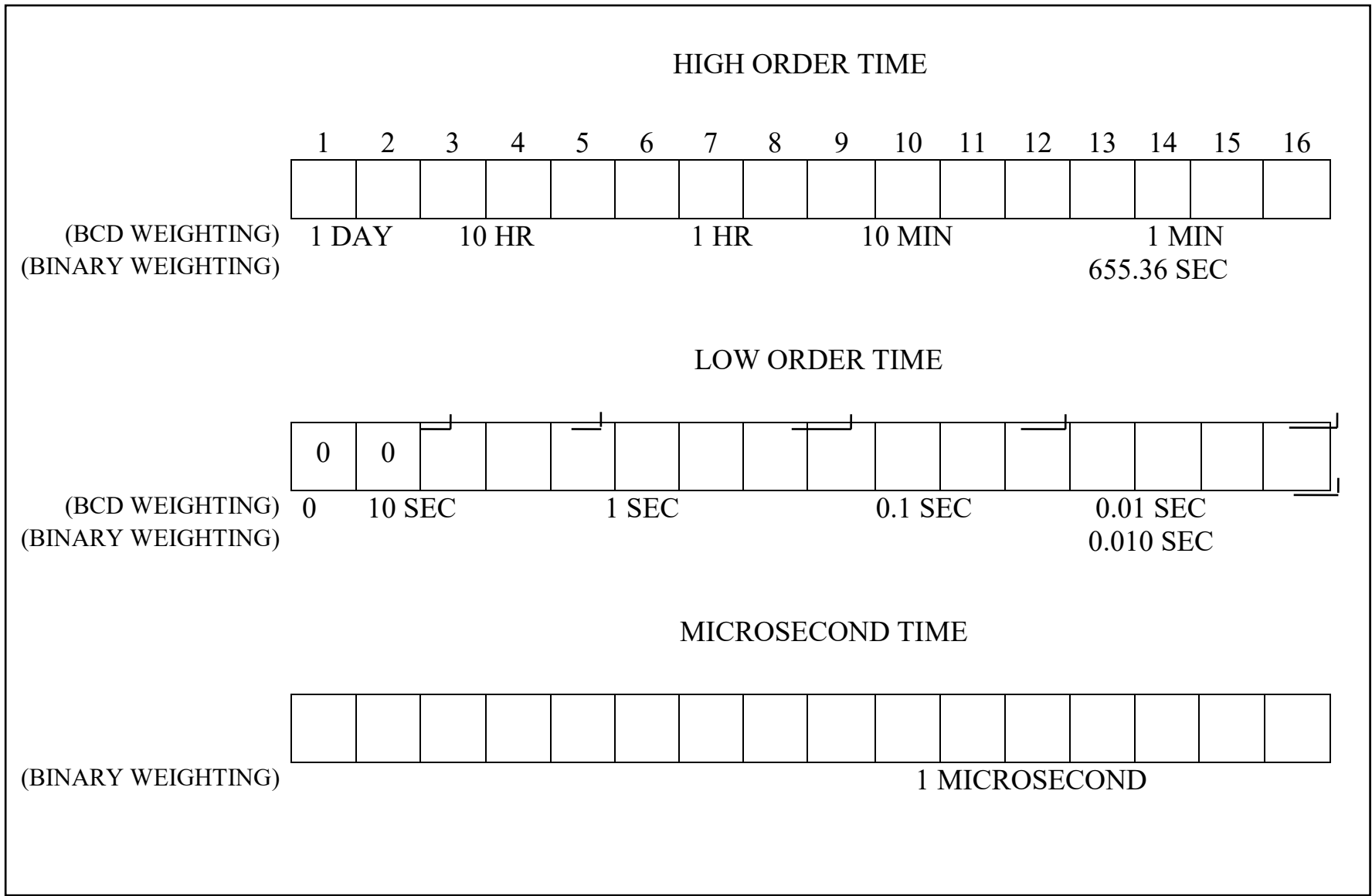
Figure 4-3. 16 bit standardized time word format.
