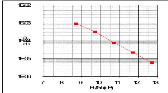
Figure A-17. FQPSK-B BEP vs E_b/N_0 .
