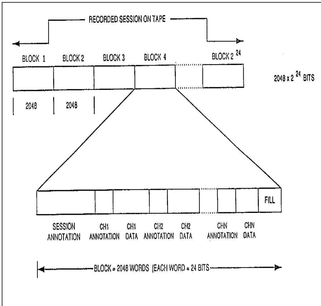
Figure 6-7. ADARIO block format.
