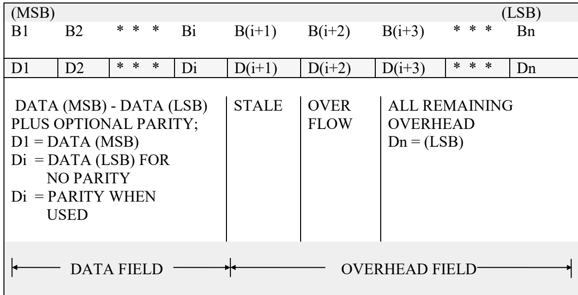
Figure 4-5. Asynchronous word structure.
