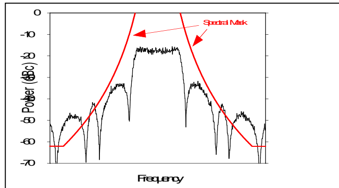
Figure A-8. Unfiltered 1-Mb/s RNRZ PCM/FM signal and spectral mask.
