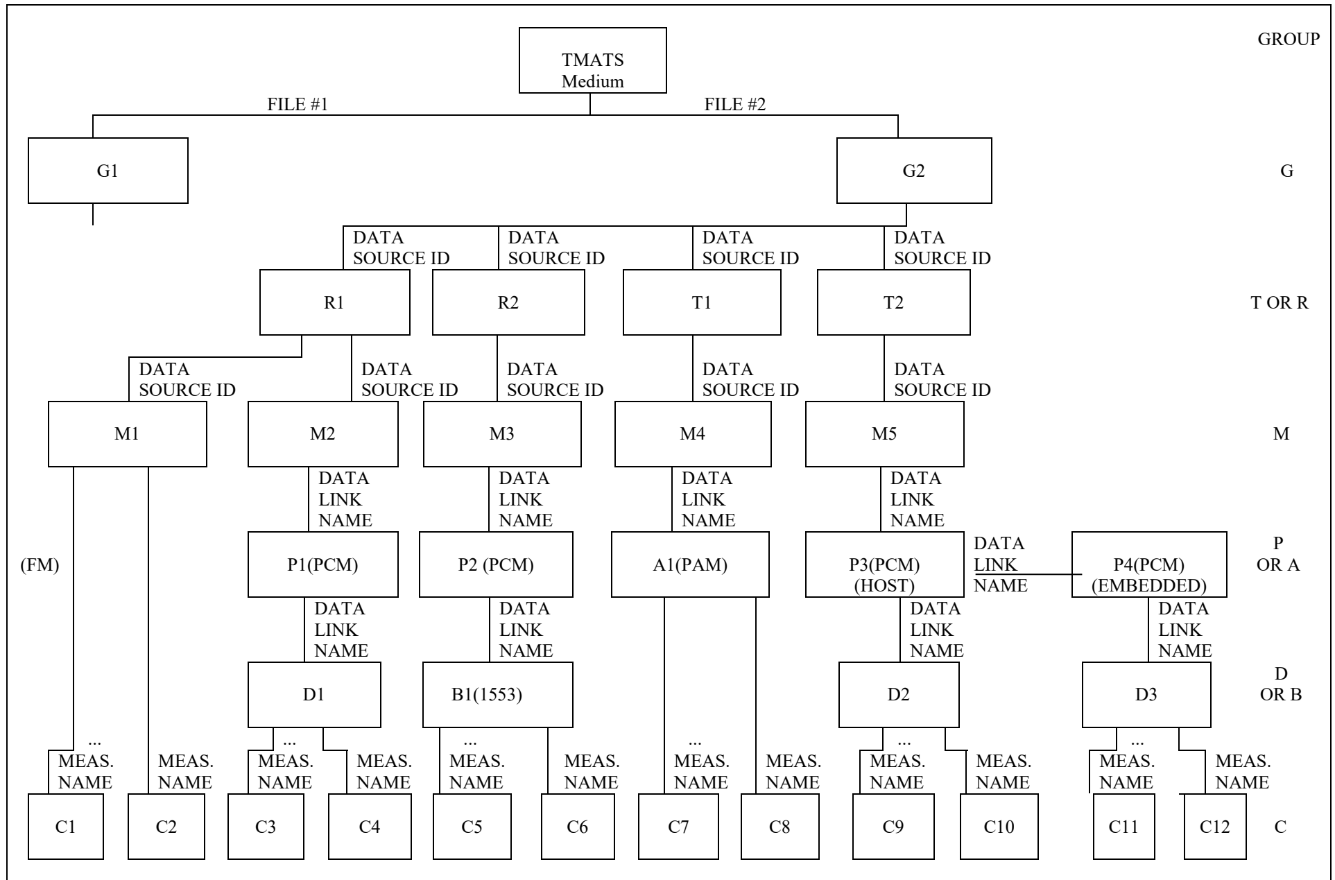
Figure 9-1. Group relationships.
