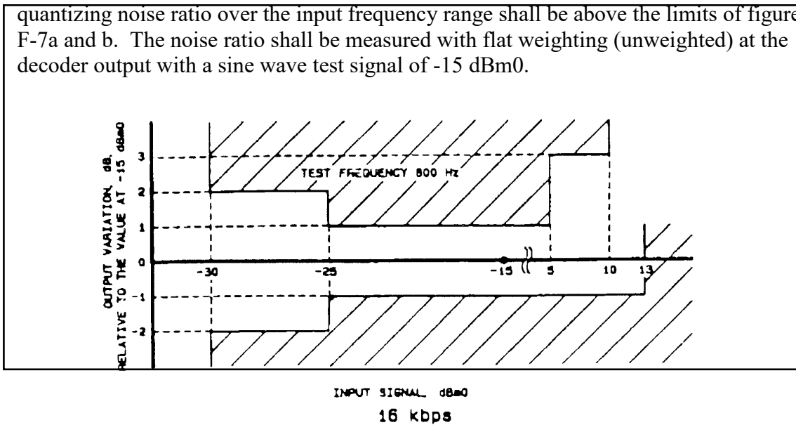
Figure F-5a. Variation of gain with input level for CVSD (16 kbps).
