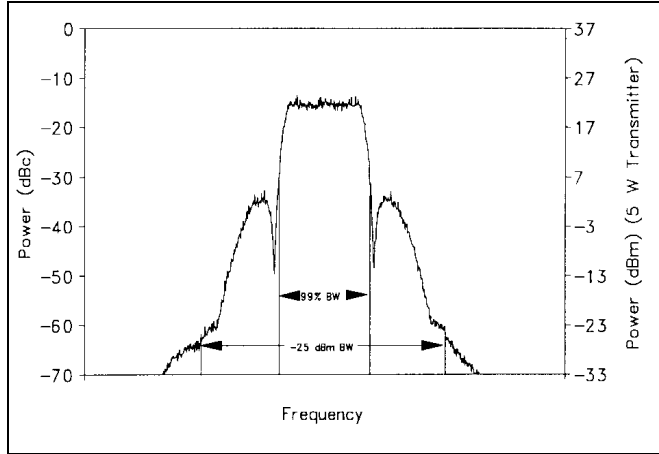
Figure A-2. 5-Mb/s NRZ PCM/FM signal
