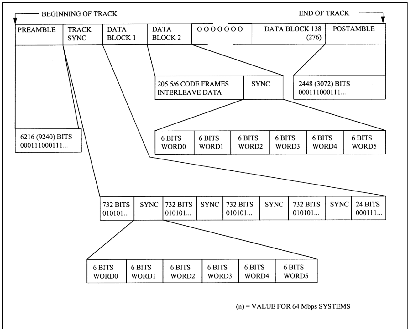
Figure 6-14. Helical Track Format.
