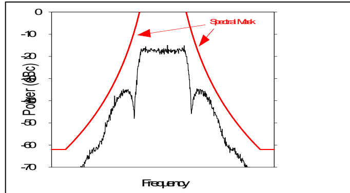
Figure A-7. Filtered 1-Mb/s RNRZ PCM/FM signal and spectral mask.
