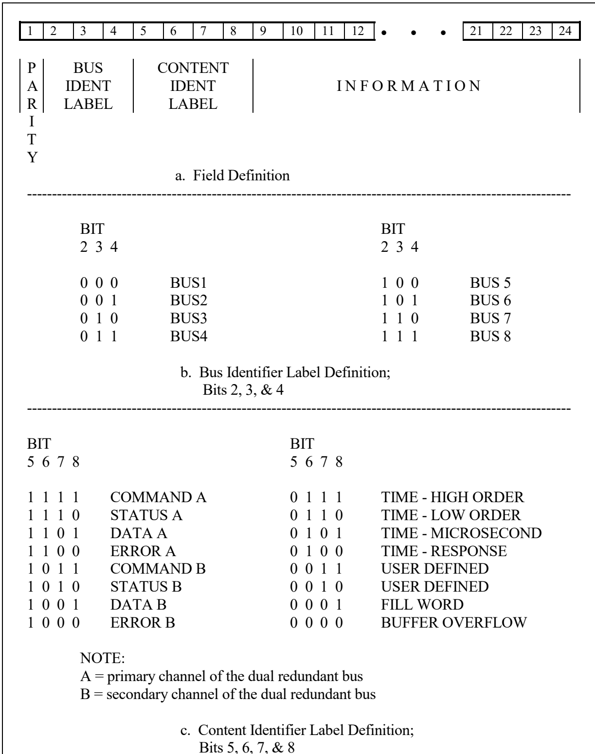
Figure 8-2. Word Construction.
