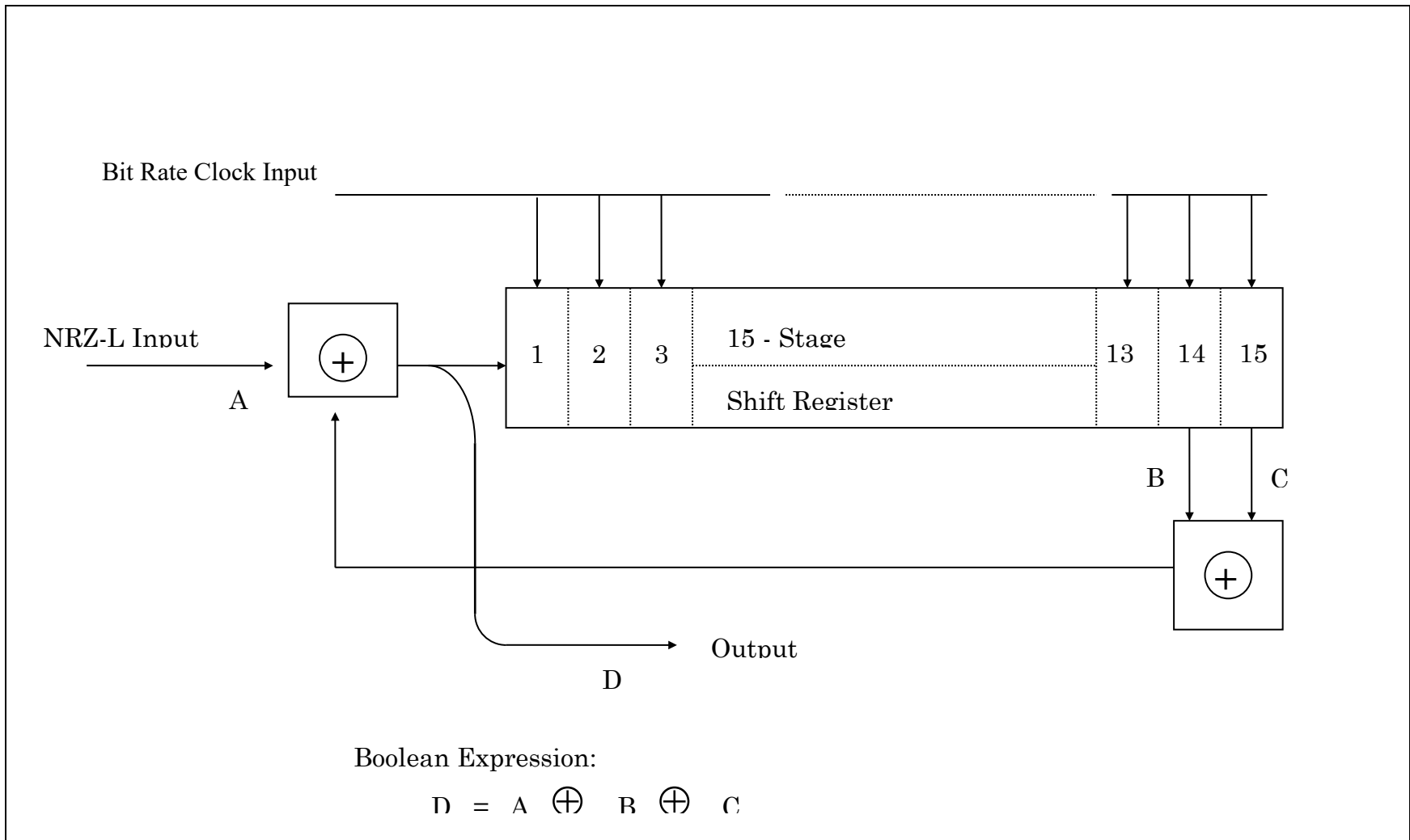
Figure D-2. Randomizer block diagram.
